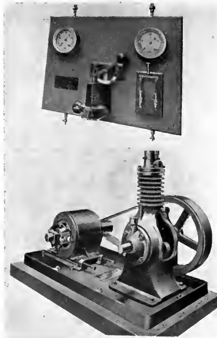
FIG. 2. MOTOR-DRIVEN AIR COMPRESSOR WITH SWITCH AND AUTOMATIC STARTING DEVICE
